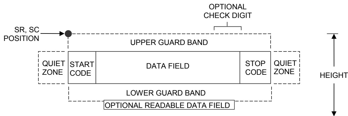
Figure 20 Telepen Structure
