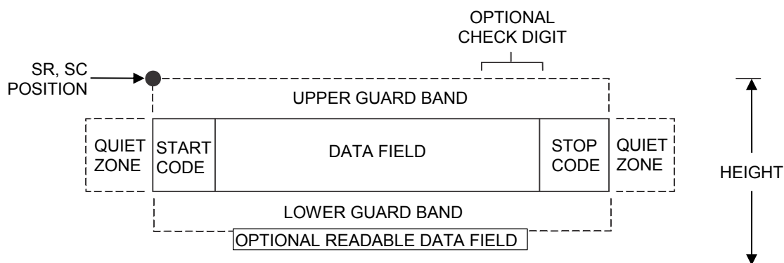
Figure 9 Code 93 Structure
