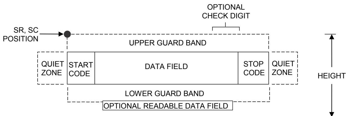
Figure 25 UPS 11 Structure
