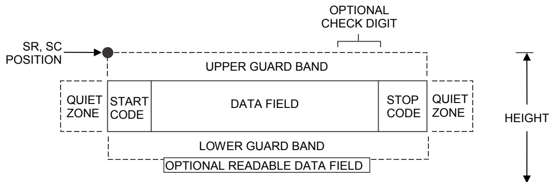
Figure 17 MSI Structure
