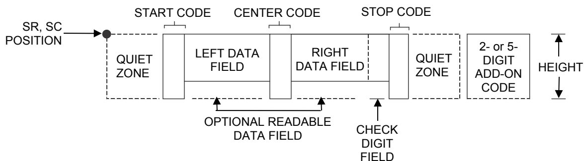
Figure 11 EAN 8 Structure
