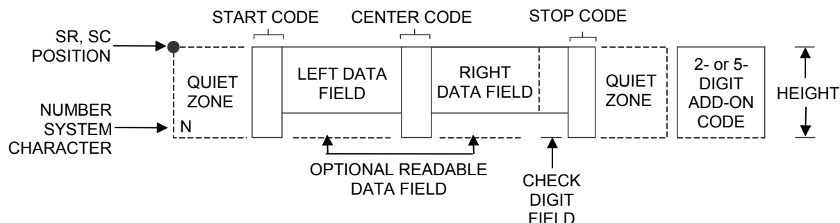
Figure 12 EAN 13 Structure
