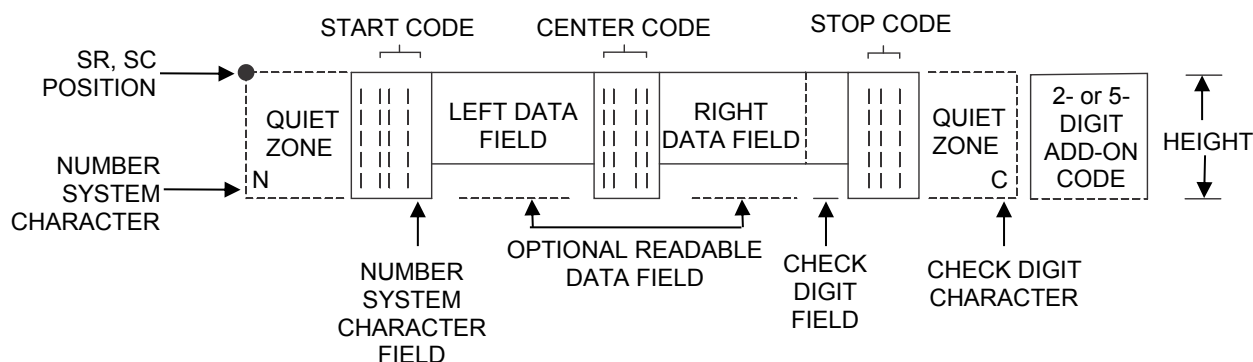
Figure 22 UPC-A Structure
