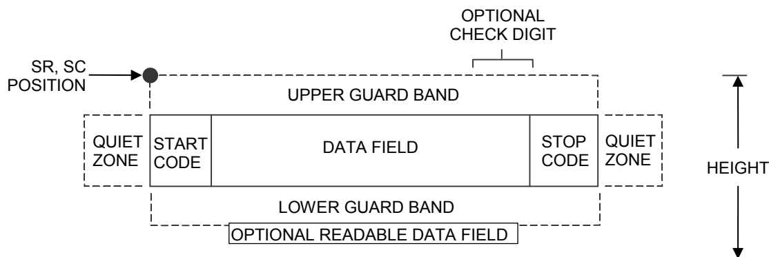
Figure 21 UCC/EAN-128 Structure
