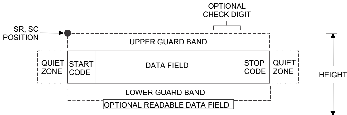
Figure 24 UPCSHIP Structure
